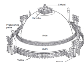
Structure outline of great stupa of Sanchi
